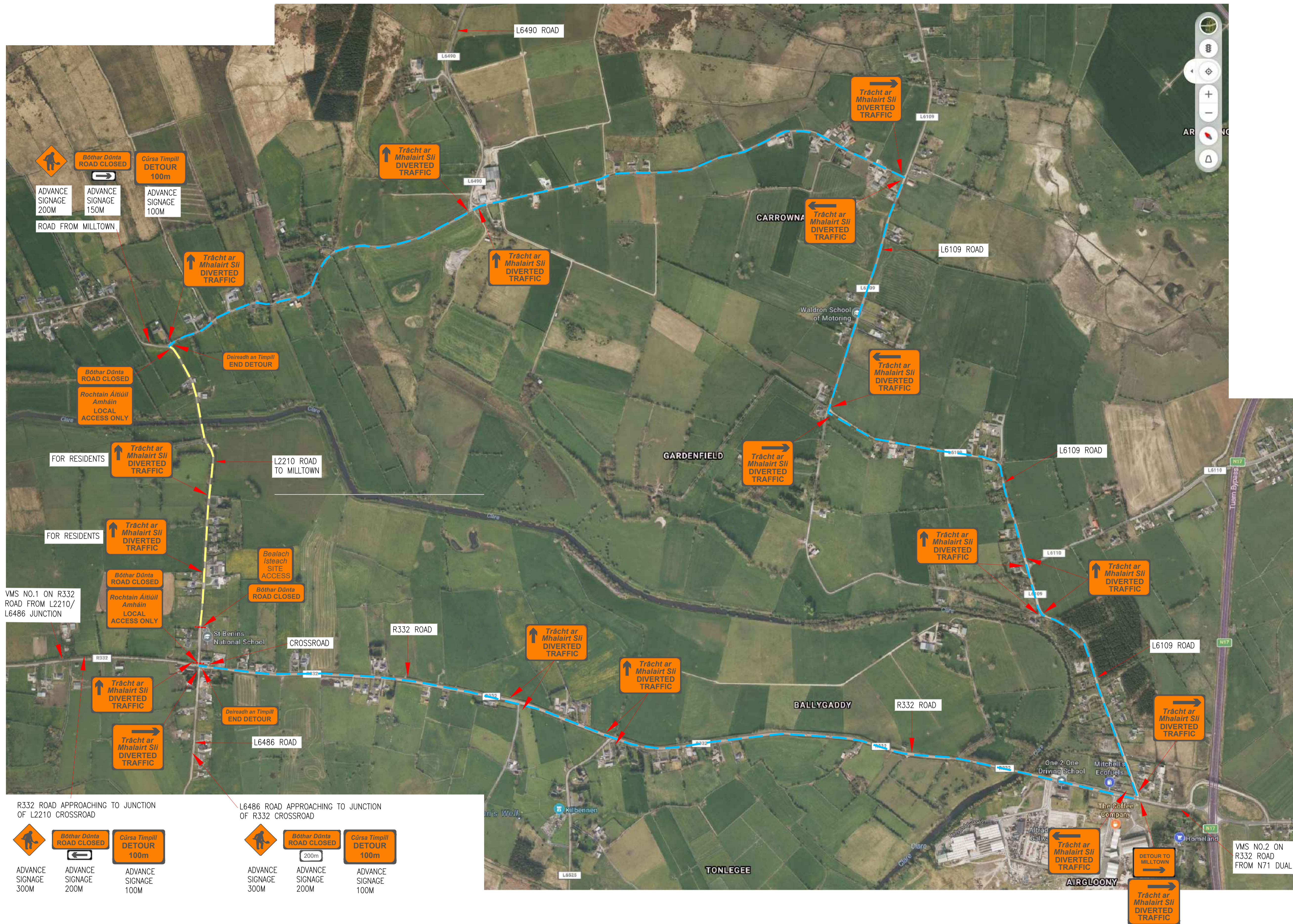
TTMP FOR L2210 ROAD (MILLTOWN) - DETOUR ROUTE
