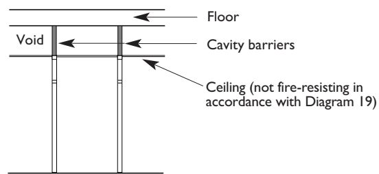
SECTION AA Cavity barriers in ceiling void over corridor walls
