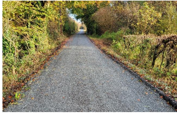
COMPLETED ROADWORKS PROGRAMME PROJECT AT CRAUGHWELL, LAURENCTOWN (L43011) USING A COLD IN-SITU RECYCLING METHOD, BEFORE & AFTER.
